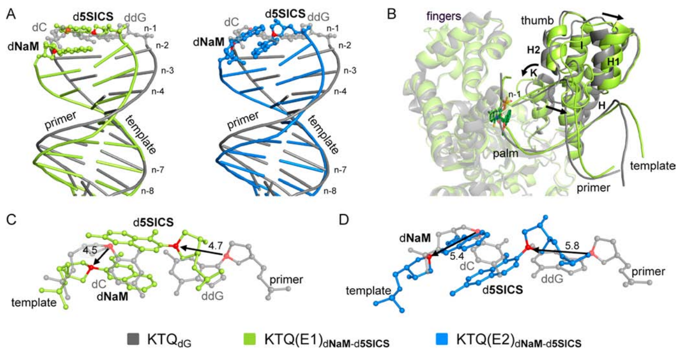
Figure 4. Comparison of \text{KTQ(E1)}_{\text{dNaM-d5SICS}} (green) and \text{KTQ(E2)}_{\text{dNaM-d5SICS}} (blue) with \text{KTQ}_{\text{dG}} with a natural dC-ddG base pair at the postinsertion site (gray). (A) Superposition of duplex portion of primer/template of \text{KTQ(E1)}_{\text{dNaM-d5SICS}} and \text{KTQ(E2)}_{\text{dNaM-d5SICS}} with \text{KTQ}_{\text{dG}} . The unnatural base pair in the postinsertion site is shown in ball and stick representation with the C1' atoms shown in red. (B) Superposition of \text{KTQ(E1)}_{\text{dNaM-d5SICS}} and \text{KTQ}_{\text{dG}} , shown as cartoon. The fingers and palm domains which are only slightly affected by the unnatural base pair are transparent. The larger movement of the thumb domain is indicated with black arrows. (C and D) Superposition of unnatural and natural base pair (from \text{KTQ}_{\text{dG}} ) at the postinsertion site with distance between C1' atoms indicated in Å, (C) \text{KTQ(E1)}_{\text{dNaM-d5SICS}} and (D) \text{KTQ(E2)}_{\text{dNaM-d5SICS}} .
